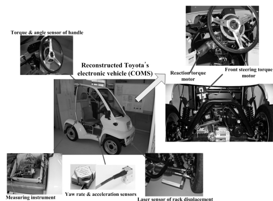
Fig. 1. Structure of SbW system.
