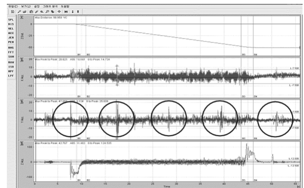
Fig. 4. Periodical vibration occurrence because of installation badness (Y axis: 25 gal).
