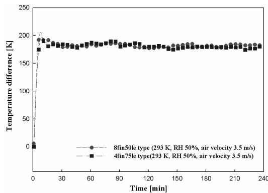
Fig. 11. Inlet-outlet temperature difference versus time of 8000mm long 8fin50le type and 4fin75le type for 4 hours experiment and constant room conditions.
