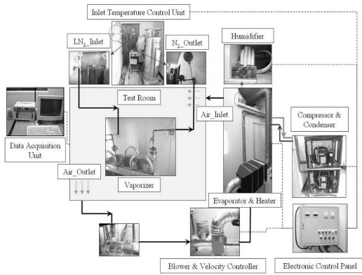
Fig. 2. Schematic diagram of experimental setup for vaporizer system.
